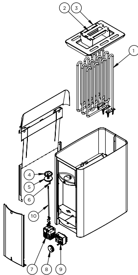
SPY10-0016 1500 W
